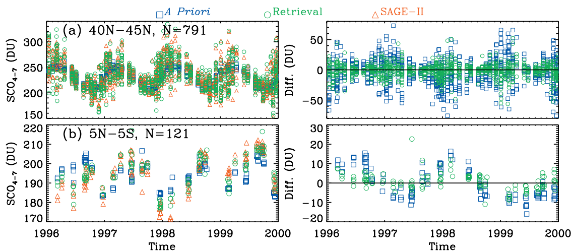
Figure 2. Comparison of Global Ozone Monitoring Experiment (GOME) retrieval/a priori and Stratospheric Aerosol and Gas Experiment II (SAGE II) column ozone over altitude range \sim 15\text{--}35 km ( \text{SCO}_{4-7} ) during 1996–1999. (left) Time series and (right) differences (GOME retrieval/a priori minus SAGE II).
