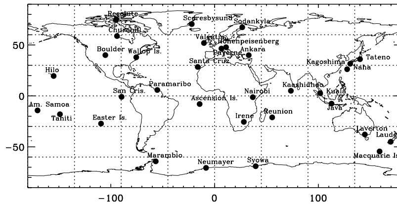
Figure 1. Locations of ozonesonde stations.
