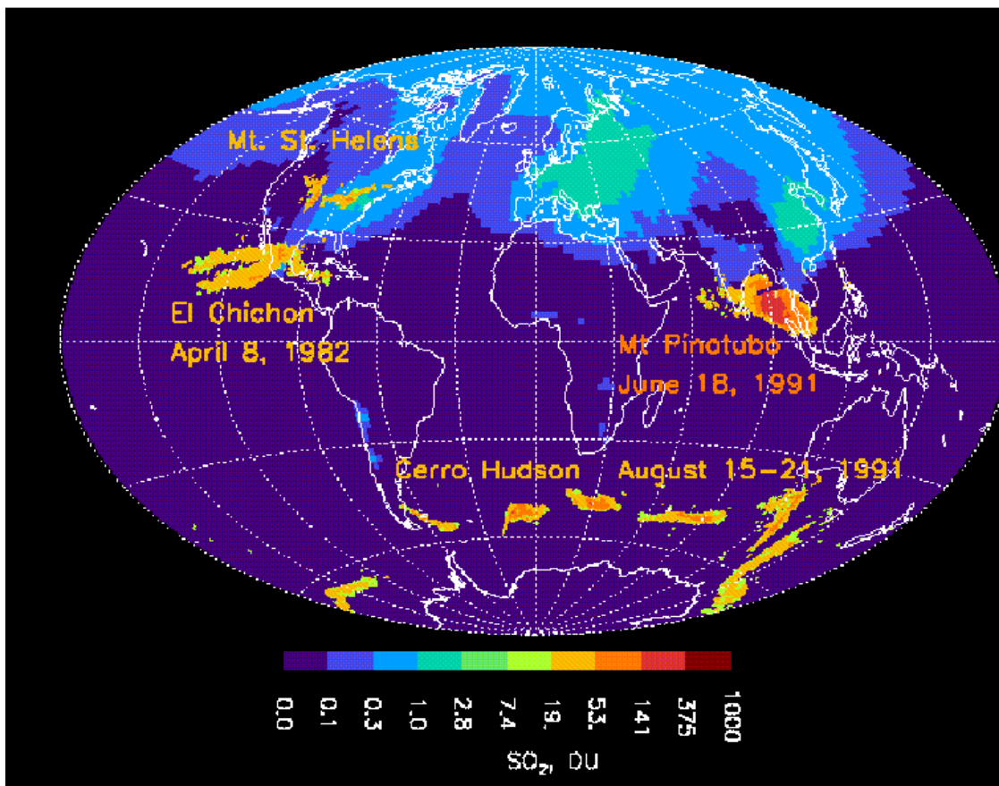
Figure 4.1 Global monthly map of air pollution SO 2 from GOCART model [Chin et al. , 2000] superimposed on global composite map of several volcanic SO 2 eruption clouds measured by TOMS [Krueger et al. , 2000].
