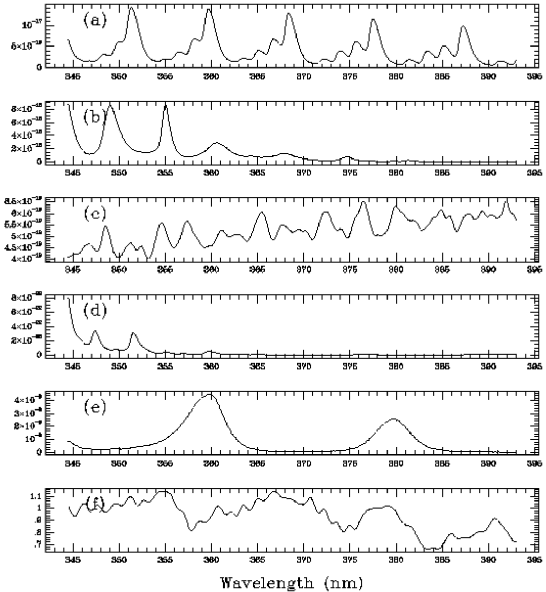
Figure 6.1 Reference spectra for fitting to determine slant column abundances of OCIO: (a) OCIO; (b) BrO; (c) NO 2 ; (d) O 3 ; (e) O 2 -O 2 collision complex; (f) Ring effect.
