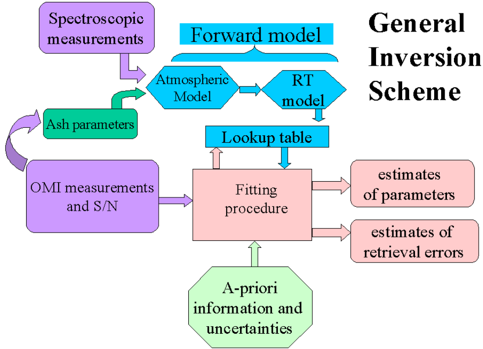
Figure 4.3 SO 2 inversion flowchart
