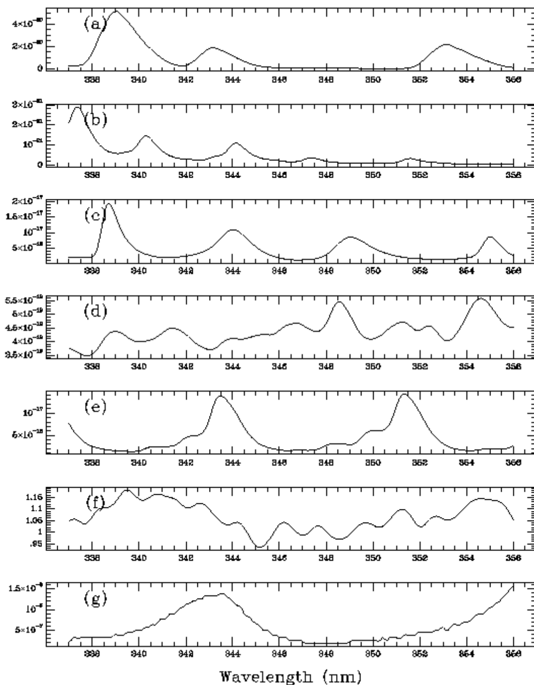
Figure 3.4 Reference spectra for fitting to determine slant column abundances of HCHO: (a) HCHO; (b) O_3 ; (c) BrO; (d) NO_2 ; (e) OCIO; (f) O_2 - O_2 collision complex; (g) Ring effect.
