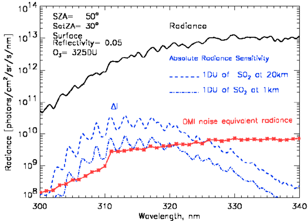
Figure 4.2 Selection of optimum wavelength region for SO 2 determination at midlatitudes with clear sky. Radiance of the midlatitude atmosphere (black curve) and differential radiance due to SO 2 layers (blue curves) compared with the noise radiance of OMI (red curve).
