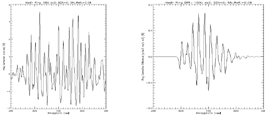
Figure 4.6 Ring correction in the SO 2 spectral fitting window: a) Standard Ring spectrum taking into account only ozone absorption and Rayleigh scattering; b) Additional correction due to 10 DU of SO 2 . A triangular slit function with a FWHM = 0.45 nm was used for this calculation.
