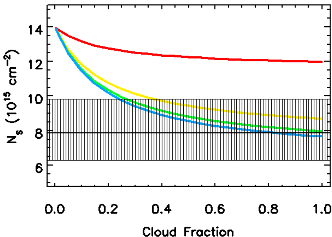
Figure 2.6 Theoretical slant column densities, N_s , vs. cloud fraction for unpolluted NO 2 and its natural variation (shaded region), and for a mixed polluted and unpolluted profile with cloud tops at 850 mb (red), 700 mb (yellow), 500 mb (green), and 200 mb (blue). The calculations assumed cloud and surface albedos of 0.80 and 0.05, respectively.
