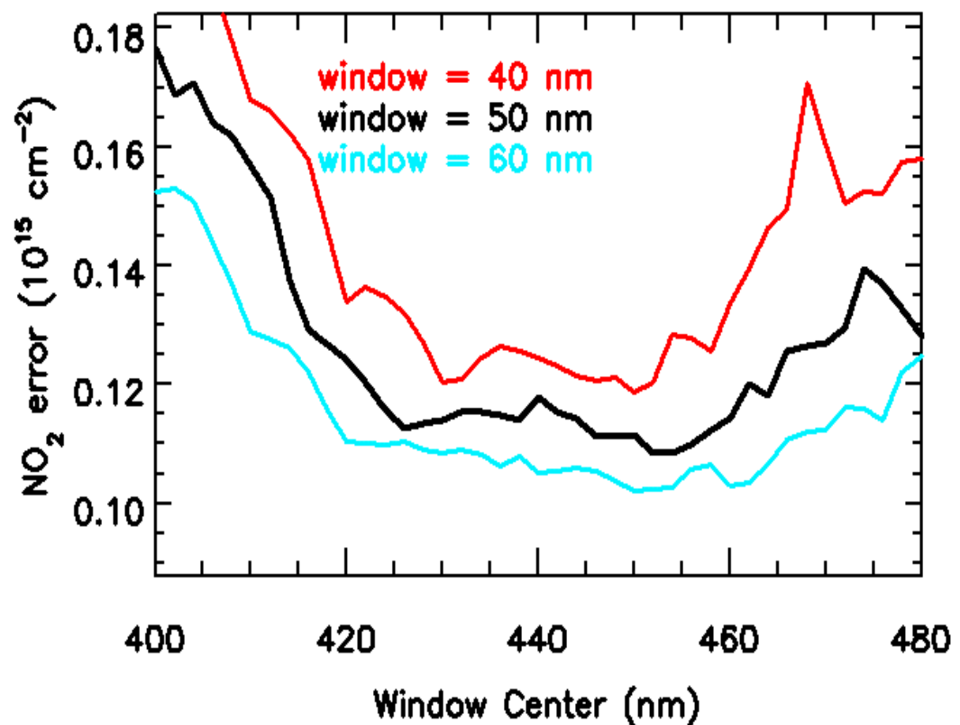
Figure 2.5 NO 2 fitting error dependence on fitting window (SNR=1000).
