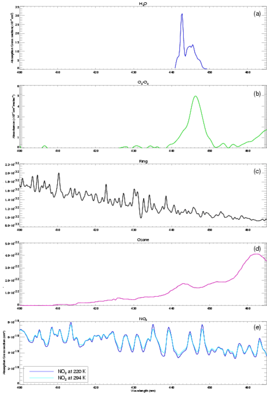
Figure 2.4 Reference spectra at OMI spectral resolution for water vapor (a), O 2 -O 2 (b), Ring effect (c), ozone (d) and NO 2 (e).
