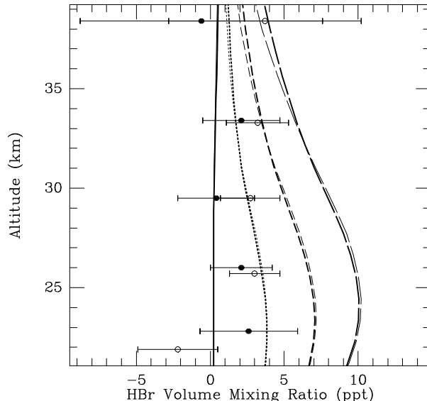
Figure 1. A comparison of the average daytime (open circles) and nighttime (solid circles) HBr mixing ratio profiles with calculated profiles A (solid), B (dotted), C (short dash), and D (long dash). Daytime average model profiles are indicated by the light lines, and nighttime averages by the heavy lines. The profile calculations are described in the text.
