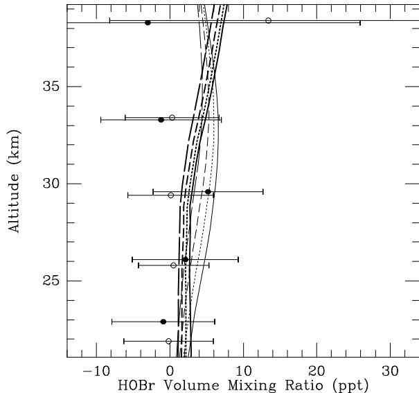
Figure 2. A comparison of the average daytime (open circles) and nighttime (solid circles) HOBBr mixing ratio profiles with calculated profiles A (solid), B (dotted), C (short dash), and D (long dash). Daytime average model profiles are indicated by the light lines, and nighttime averages by the heavy lines. The profile calculations are described in the text.
