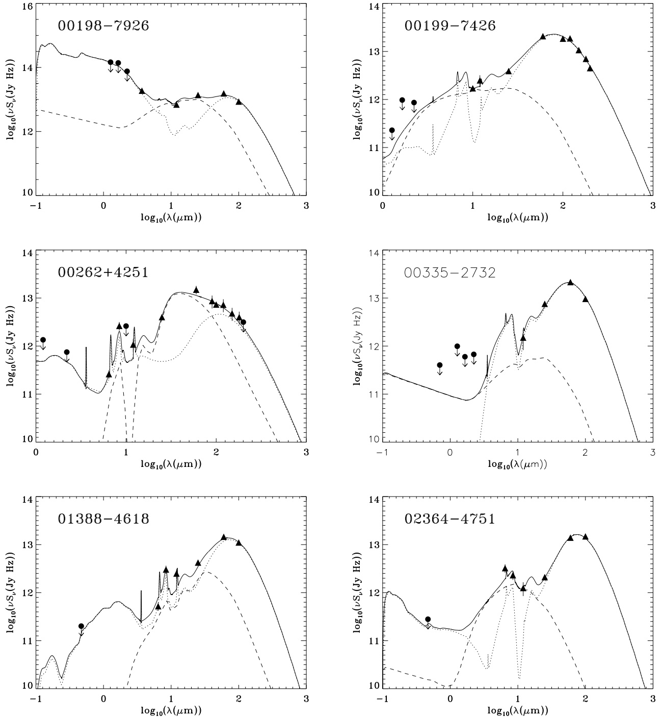
Figure 1. Best fit Spectral Energy Distributions for the 41 ULIRGs in our sample. In each case the solid line is the combined best-fit model, the dotted line is the Starburst component and the long dashed line is the AGN component.
