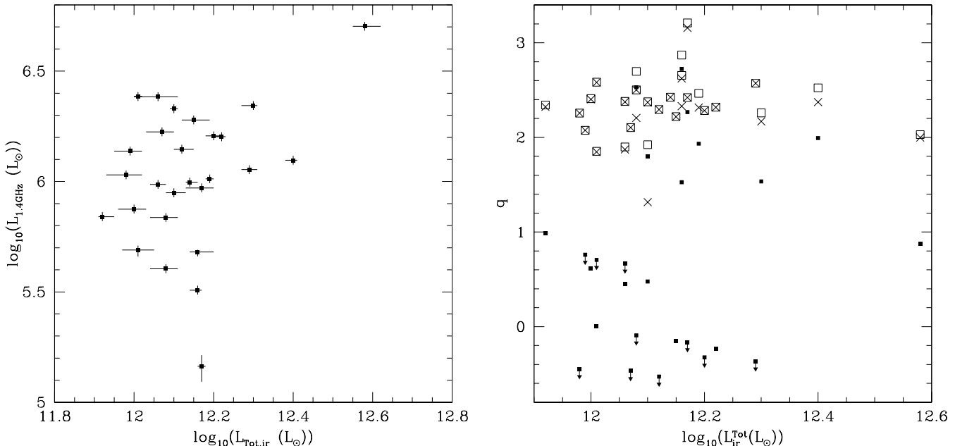
Figure 6. (Left) Total IR luminosity plotted against total radio luminosity. (Right) Total IR luminosity vs. q parameter. Open squares are q_{\text{total}} , crosses are q_{\text{starburst}} , and small filled squares are q_{\text{AGN}} . A downward arrow indicates an upper limit.
