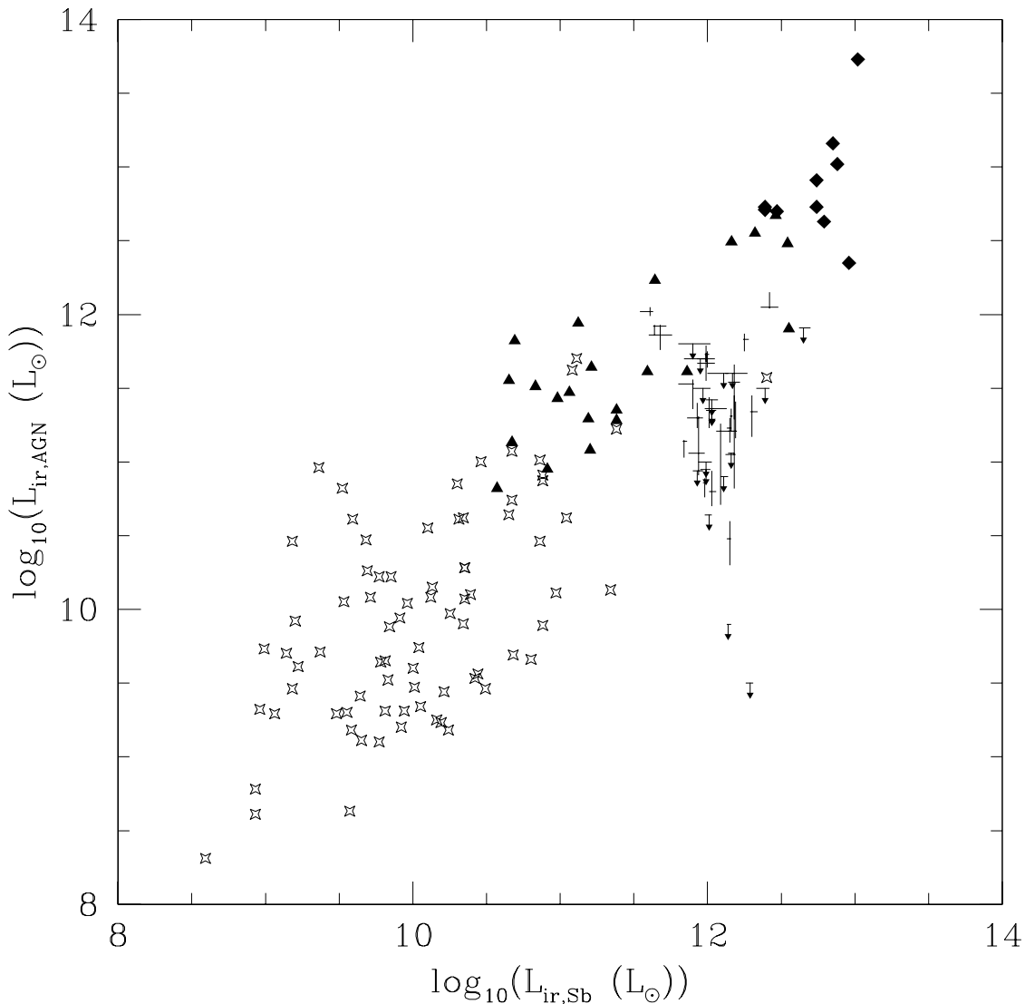
Figure 2. AGN luminosity in the IR plotted against starburst luminosity in the IR. The ULIRGs from our sample are plotted as points, with a downward arrow indicating an upper limit on the AGN luminosity. Triangles are PG QSOs, and crosses are those galaxies with detections in all four IRAS bands, both these samples are taken from Rowan-Robinson (2000). Diamonds are the Hyperluminous Infrared Galaxies taken from Farrah et al (2002b).
