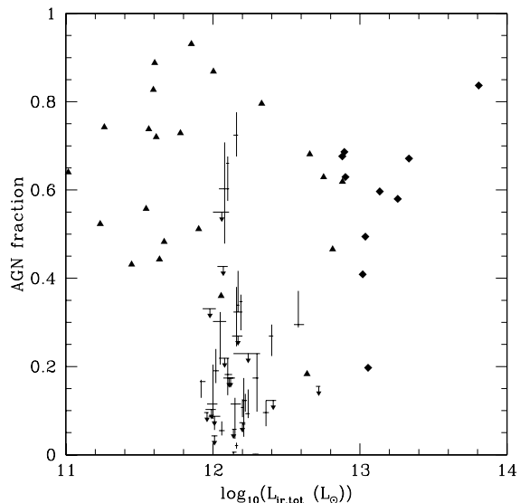
Figure 4. Total luminosity in the IR plotted against AGN fraction. Key to the symbols is the same as for Figure 3
