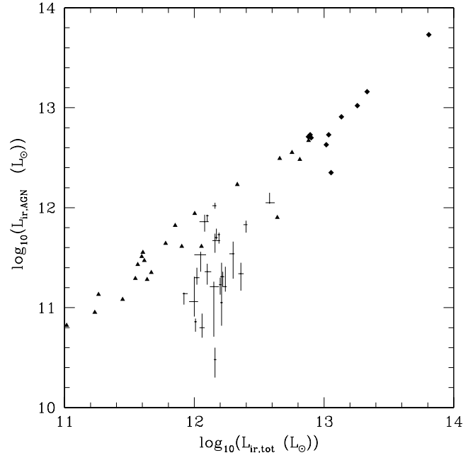
Figure 3. Total IR luminosity plotted against (left) starburst luminosity and (right) AGN luminosity. Our ULIRGs are plotted as points, triangles are PG QSOs taken from Rowan-Robinson (2000), and diamonds are the HLIRGs from Farrah et al (2002b)
