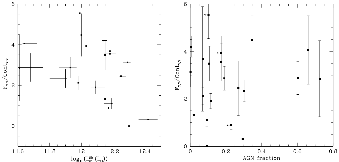
Figure 5. (Left) Starburst luminosity plotted against 7.7\mu\text{m} line/continuum ratio from Rigopoulou et al (1999). (Right) Fractional AGN luminosity plotted against 7.7\mu\text{m} line/continuum ratio
