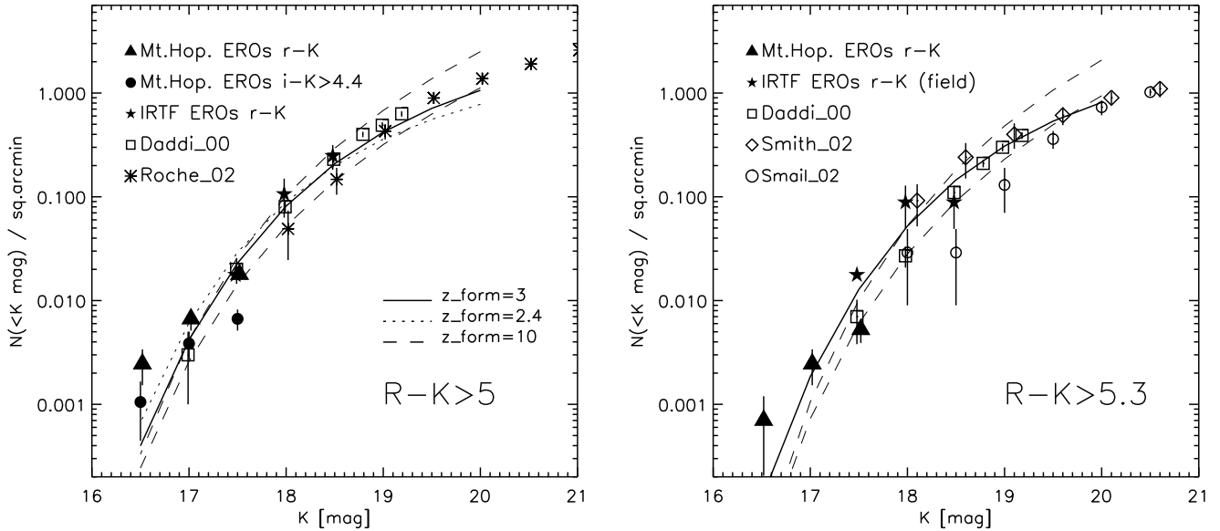
Fig. 7. Cumulative ERO counts are shown for R - K > 5 and R - K > 5.3 selections (ie. r - K > 5.5 and r - K > 5.8 ), in the left and right panels, respectively, with solid triangles. Additionally, the i - K > 4.4 selected EROs are plotted in the left panel with circles. Error bars are Poissonian. Our other field ERO counts from a deeper survey (IRTF, Väisänen & Johansson 2004) are shown as stars. Squares show the EROs of Daddi et al. (2000a) and the asterisks the Roche et al. (2002) EROs in the left panel. The left panel shows R - K > 5 selected EROs of Daddi et al. (2000a) and Roche et al. (2002). In addition to the Daddi et al. R - K > 5.3 selected EROs the right panel plots the corresponding Smith et al. (2002) and Smail et al. (2002) EROs. We plot PLE models of Daddi et al. calculated using the indicated R - K cuts. The curves are different by their galaxy formation redshifts, as indicated in the figure. The two dashed-lines employ a different LF – the higher curve results from a 2MASS normalized LF, and the lower from that of Marzke et al. (1994).
