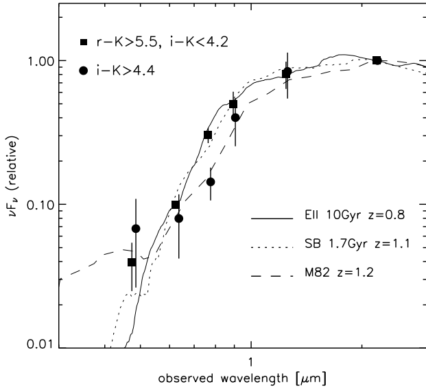
Fig. 6. Averaged and K -band normalized SEDs of i - K EROs (circles) and those r - K EROs with i - K < 4.2 (squares). The observed bands are g, r, i, Z, J, K . The GRASIL M82 model and elliptical and evolved starburst SEDs from BC are also plotted at indicated redshifts.
